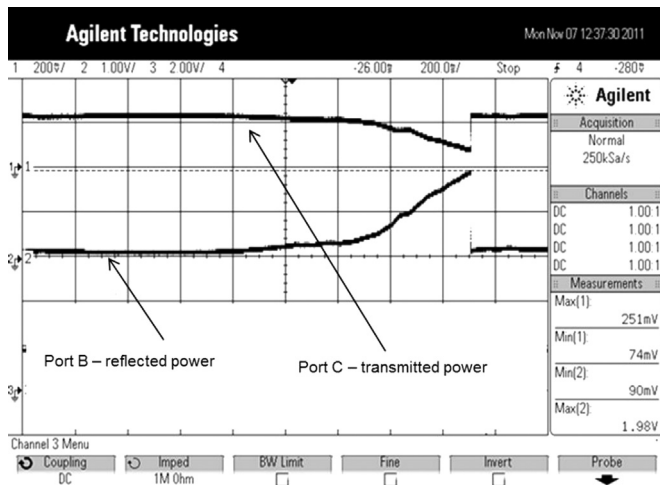
Fig. 2. Typical oscilloscope traces for transmitted and reflected powers at critical coupling regime.
