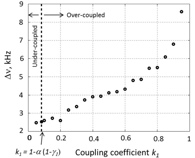
Fig. 6. Linewidth of the locked DFB laser versus coupling factor k_1 .
