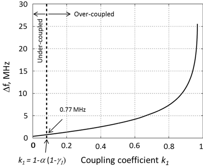
Fig. 4. Linewidth of the resonance mode of FORR versus coupling factor k_1 .
