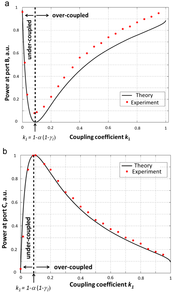
Fig. 3. Reflected (a) and transmitted (b) powers versus coupling coefficient k_1 .
