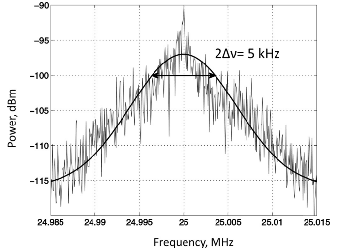
Fig. 5. Delayed self-heterodyne spectra of the locked DFB laser for the critical coupling.
