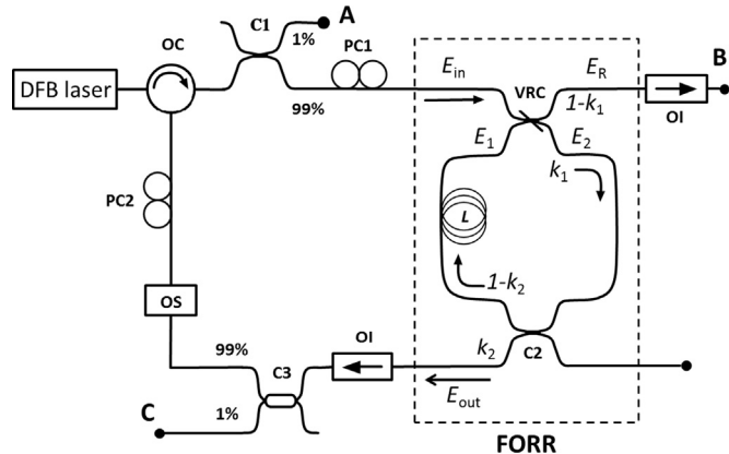
Fig. 1. The experimental configuration; OC – optical circulator, PC – polarization controller, C – coupler, OI – optical isolator, OS – optical switcher, VRC – variable ratio coupler, and FORR – fiber-optic ring resonator.
